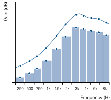
Vérité’s ChannelFree™ DSP allows precise independent gain adjustments, while keeping the response smooth across the frequency range
